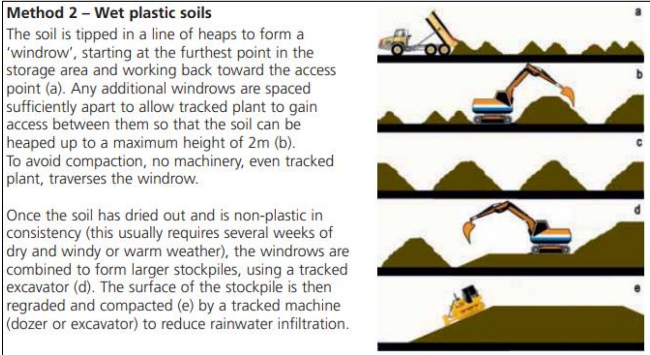
Figure F.2 - Wet plastic soil stockpile technique (Defra , 2009 )
