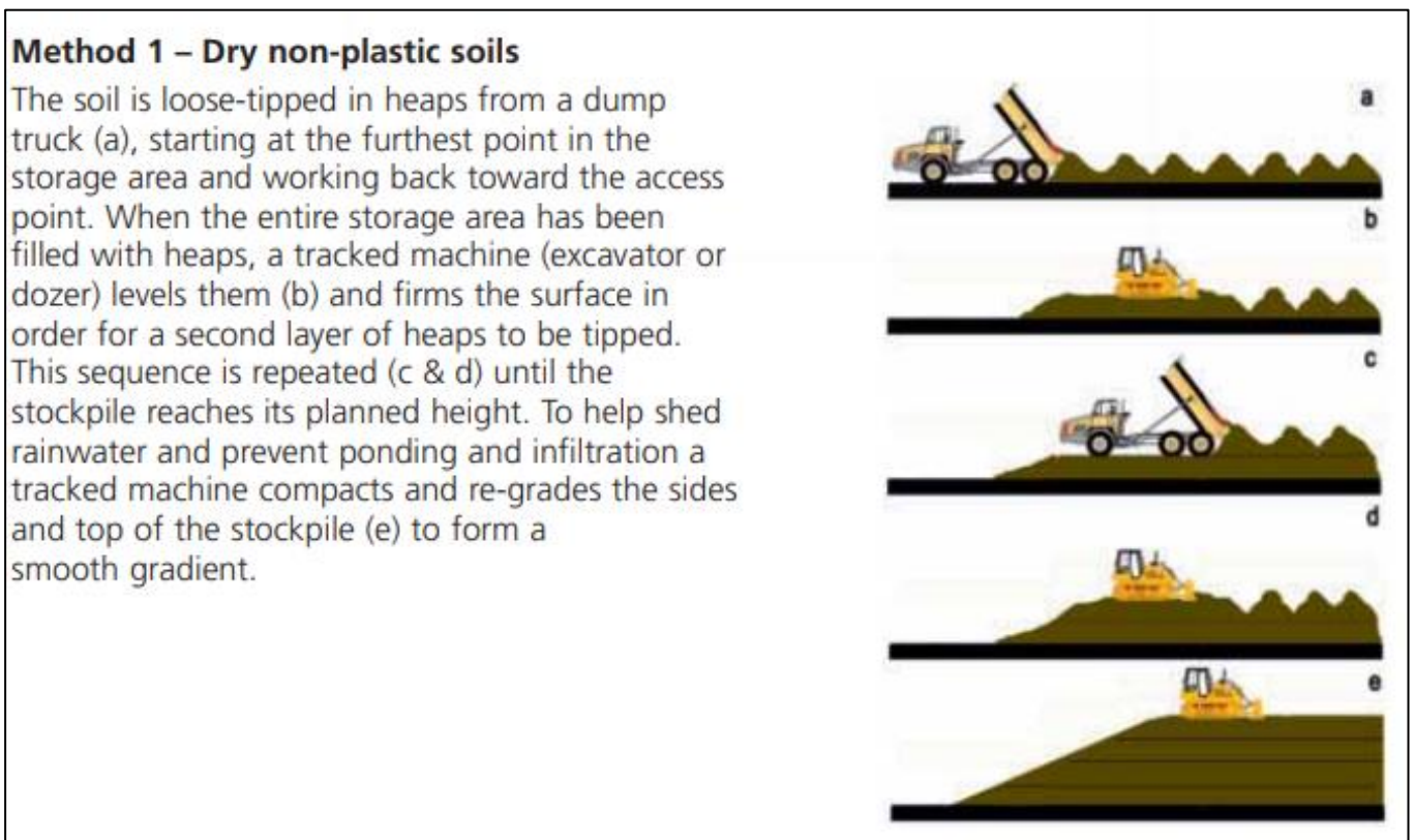
Figure F.1 - Dry non-plastic soil stockpile technique (Defra , 2009 )
